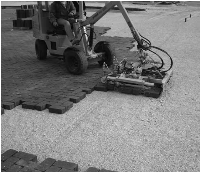
Figure 27 and 28. Mechanical equipment accelerated installation of a parking lot in Illinois and a street in Oregon.
