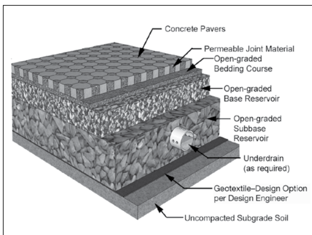
Figure 1. PICP typical cross section.
